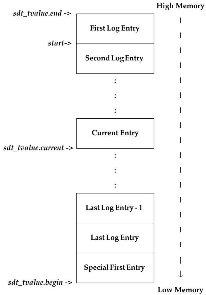
Figure 5-1. Debug Trace Memory Structure
